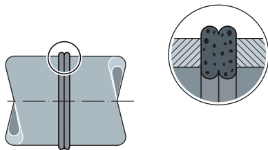
Jointing fault (external finding) – fusion bead with bubbles
