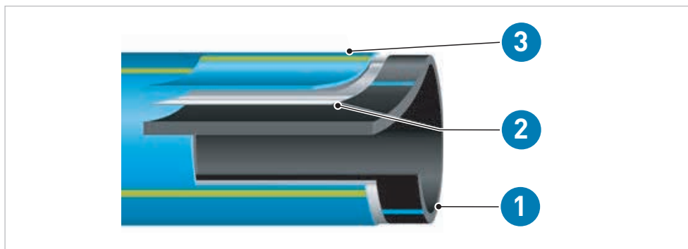
Layer buildup of pipes with diffusion barrier
