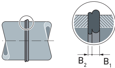
Jointing fault (external finding) – unequal fusion bead
