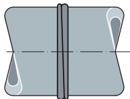
Jointing fault (internal finding) – lack of adhesion
