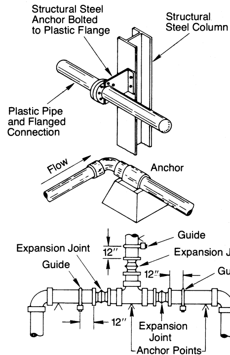
Figure 4-15: A typical method of anchorage of a change in direction
