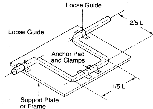
Figure 4-15: A typical method of anchorage of a change in direction
