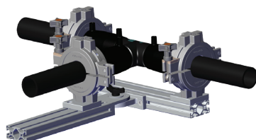
Tee Kit
