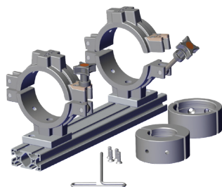
Standard Kit
